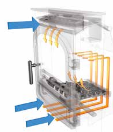
INSET AIRFLOW
